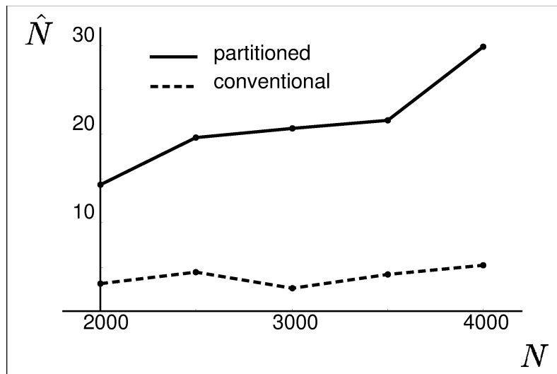
Figure 15: Estimated effective sample size \hat{N} for partitioned and conventional (unpartitioned) sampling methods. The graph shows the average value of \hat{N} following a 10-frame sequence tracking two leaves. Note the superior performance of the partitioned sampling method.
