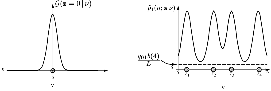
Figure 3: 1-target likelihood function for a single measurement line. Left: The boundary feature distribution \mathcal{G}(z = 0|\nu) . Right: The 1-target likelihood function \tilde{p}_1(n; \mathbf{z}|\nu) graphed with respect to \nu . The likelihood is a linear combination of shifted copies of \mathcal{G}(z|\cdot) and of the constant p_0 . It peaks near the 4 measurements z_i (shown as shaded circles).
