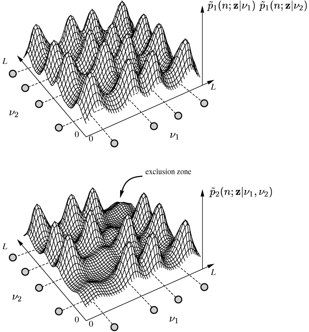
Figure 4: 2-target likelihood functions for a single measurement line. Top: A naïve 2-target likelihood \tilde{p}_1(n; \mathbf{z}|\nu_1)\tilde{p}_1(n; \mathbf{z}|\nu_2) formed by taking the product of two 1-target densities (figure 3). The likelihood peaks near pairs of measurements z_i, z_j (shaded circles and dotted lines). Bottom: The 2-target likelihood \tilde{p}_2(n; \mathbf{z}|\nu_1, \nu_2) derived from the generative model. Again, the likelihood peaks near pairs of measurements z_i, z_j (shaded circles and dotted lines), but now a probabilistic exclusion principle operates: because the sum in the definition of p_2 excludes i = j , the probability peaks are much smaller on the line \nu_1 = \nu_2 .
