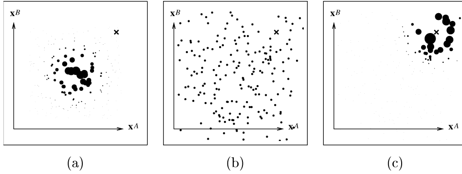
Figure 12: Conventional (i.e. non-partitioned) Condensation. The true position of the target in this 2-dimensional configuration space is shown as a cross; particles representing a probability distribution are shown as circles whose areas are proportional to their weights. Each step shown is one stage in the condensation diagram (4). (a) The prior. (b) After the dynamics have been applied. (c) After reweighting by the posterior. The posterior is centred at approximately the correct position, but this representation of the posterior is not very accurate because relatively few particles have significant weights. In technical terms, the estimated effective sample size (10) is low. Superior results are achieved using partitioned sampling (figures 13 and 14).
