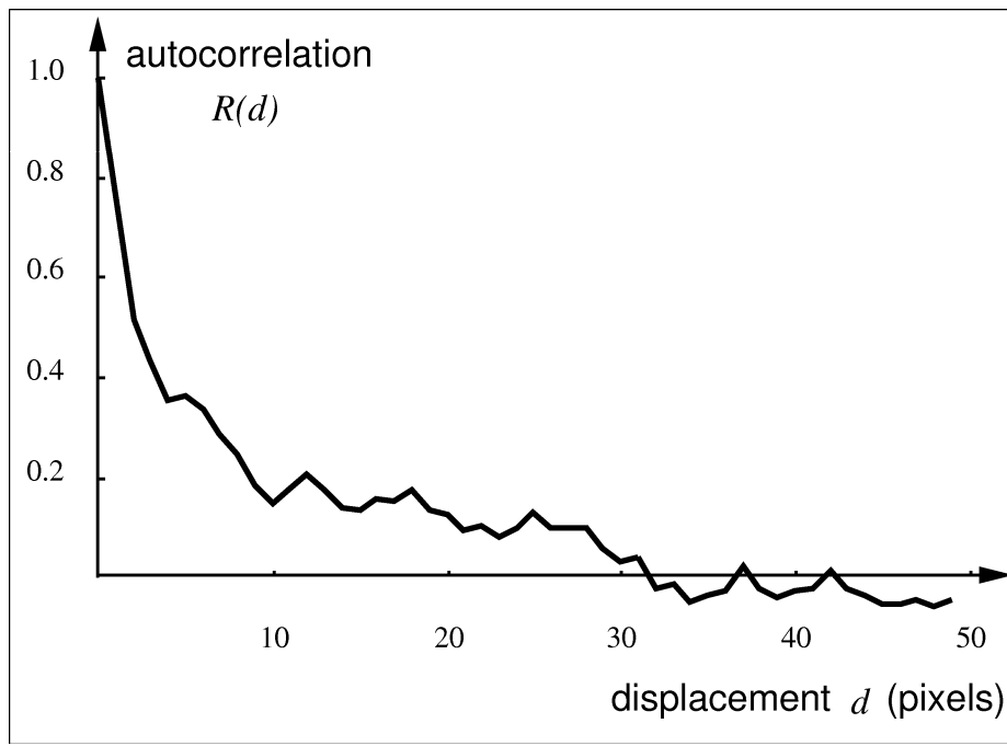
Figure 5: Feature autocorrelation is low for displacements of more than 30 pixels. This is our justification for treating distinct measurement lines as statistically independent. The random process x(d) whose autocorrelation is graphed here is described in the text and figure 6, and the autocorrelation function is defined as usual by R(d) = (E[x(d)x(0)] - E[x(0)]^2) / (E[x(0)^2] - E[x(0)]^2) .
