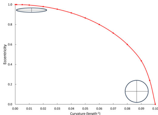
Figure 3. Graph showing how curvature across an elliptical branch decreases with increasing eccentricity. Insets show transverse sections through endmember elliptical branches.
