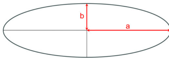
Figure 2. Geometry of an ellipse showing the semi-major ( a ) and semi-minor ( b ) axes.
