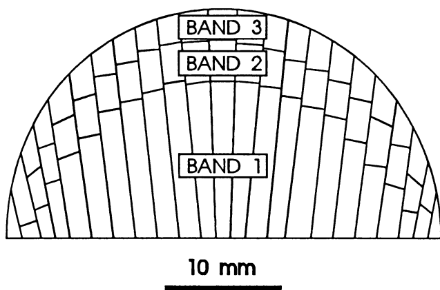
FIGURE 1. Generalized longitudinal section of a Prasopora colony showing internal band stratigraphy. Modified from Mannil (1961, fig. 1a).
