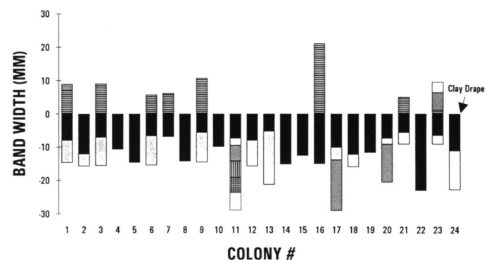
FIGURE 7. Correlation of bands (in mm) assuming an isochronous clay drape.
