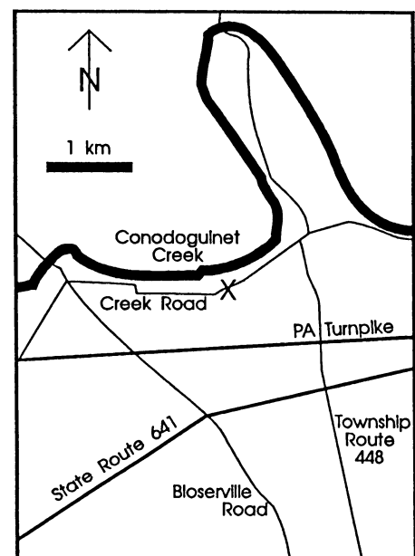
FIGURE 2. Map showing collection location marked by X.
