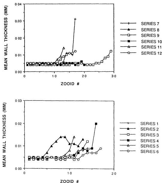
FIGURE 3. Relationship between mean zoecial wall thickness and zooid number for the six Ordovician series (bottom) and the six Devonian species (top). Series numbers refer to Table 1.
