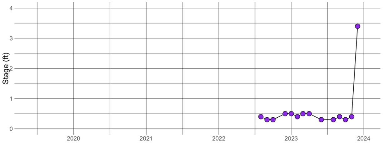
DEECRE38.64 - Stage
