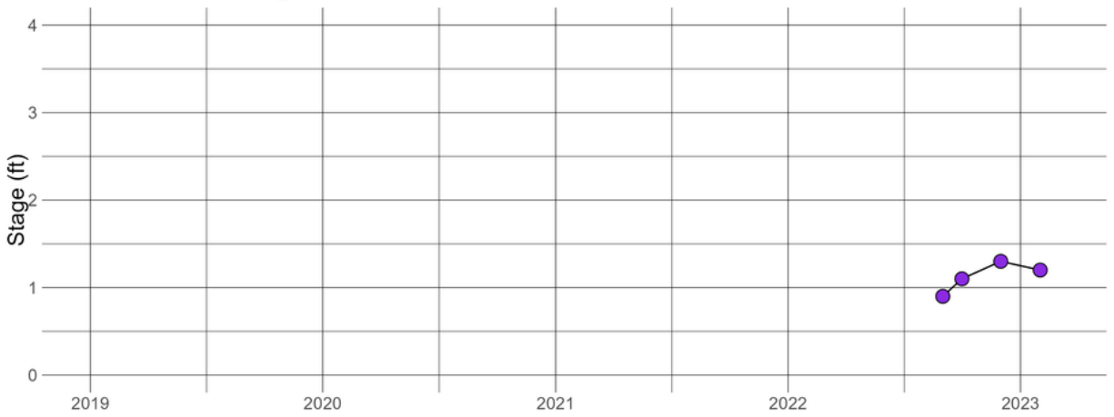
CENCRE0.07 - Stage
