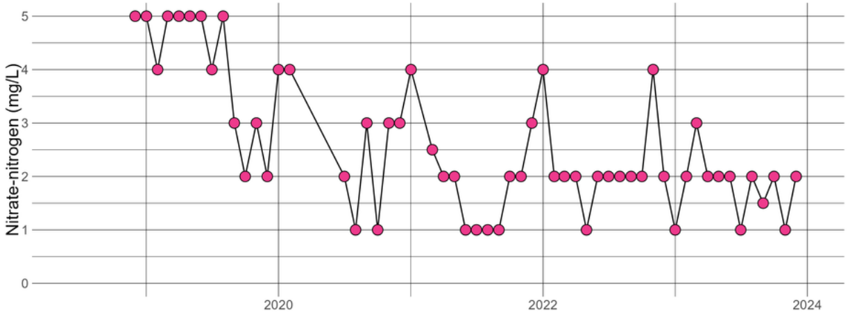
TYLRUN0.50 - Nitrate-nitrogen
