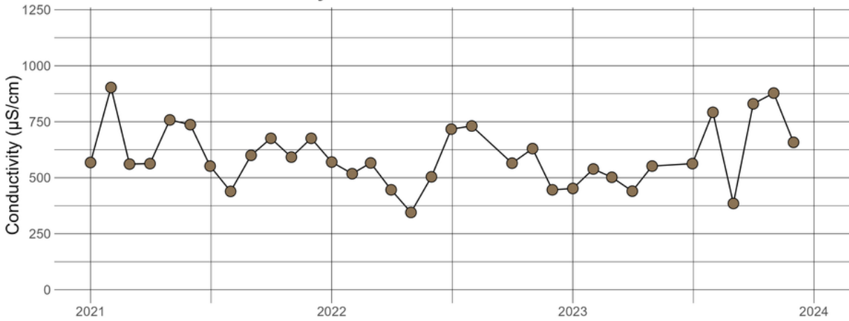
CODCRE5.77 - Conductivity
