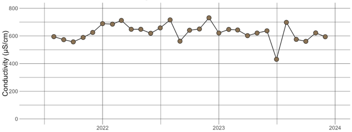
UNTCODCRE1.28 - Conductivity
