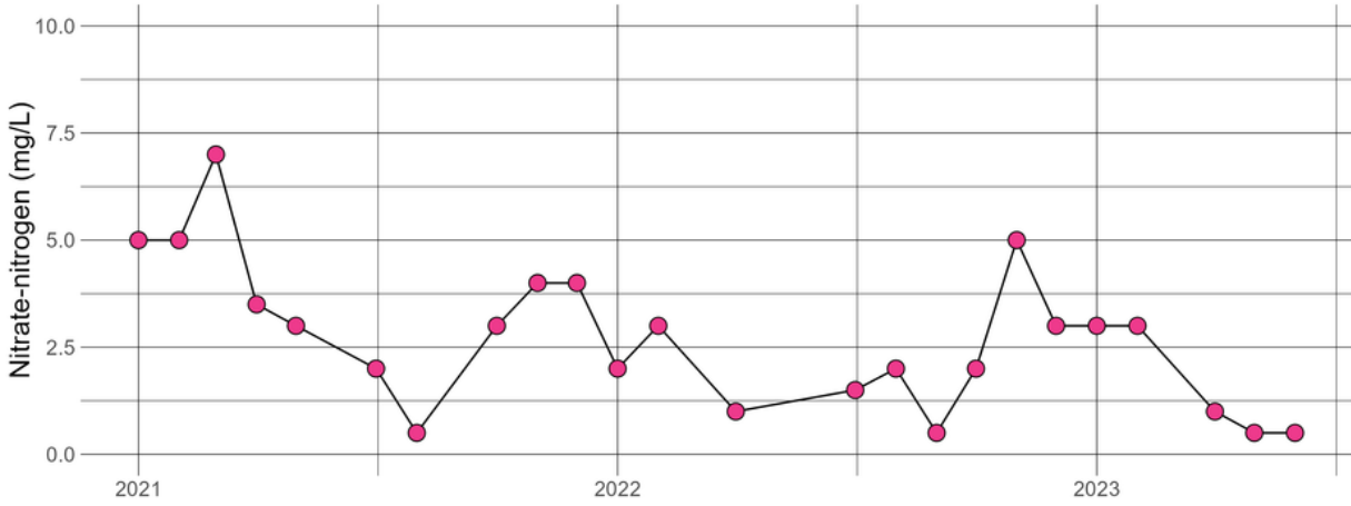
SOUBRACODCRE23.11 - Nitrate-nitrogen
