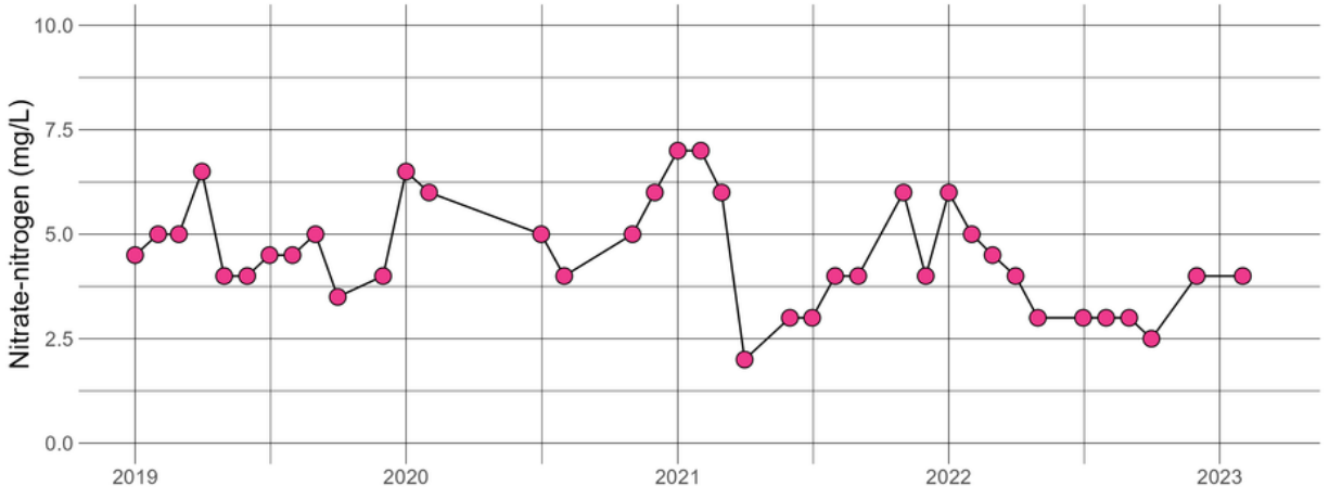
CENCRE0.07 - Nitrate-nitrogen
