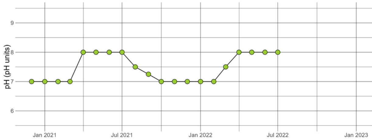
EASBRACODCRE24.60 - pH
