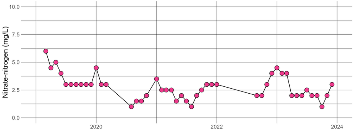
CODCRE12.39 - Nitrate-nitrogen
