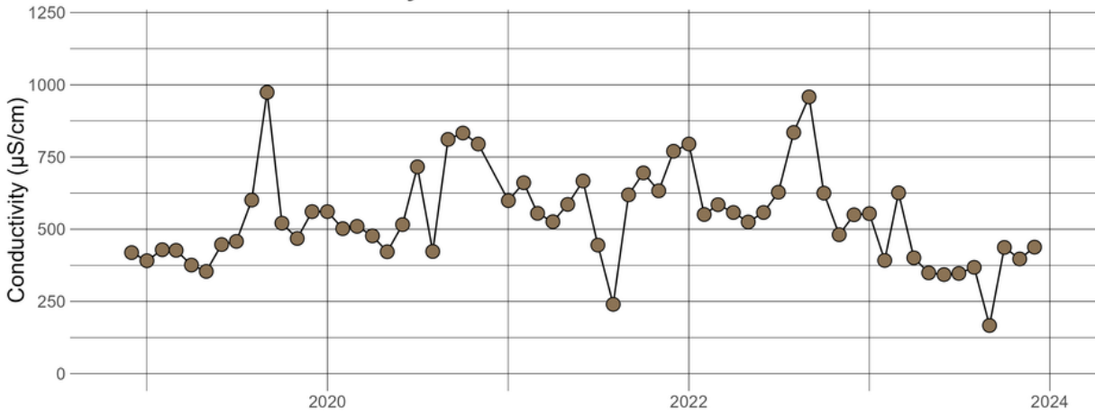
KRECRE8.67 - Conductivity
