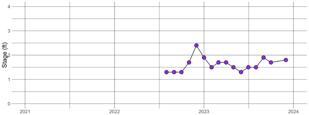
MUDCRE17.55 - Stage
