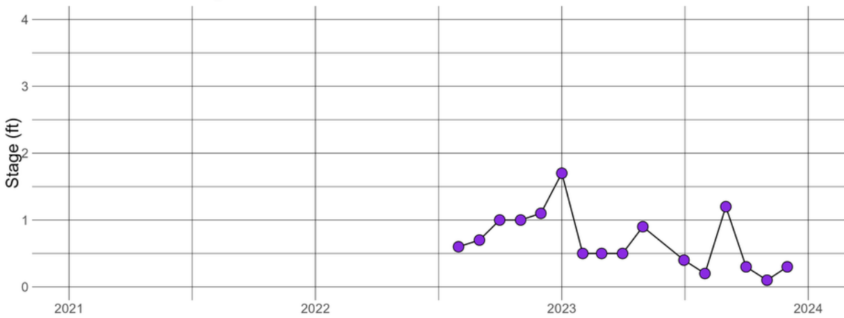
CODCRE5.77 - Stage
