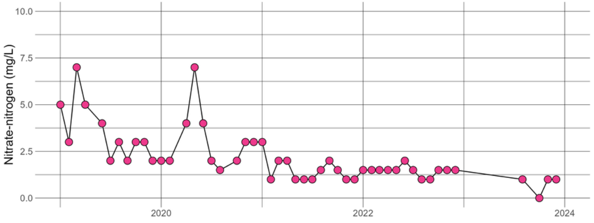
MILCRE0.09 - Nitrate-nitrogen
