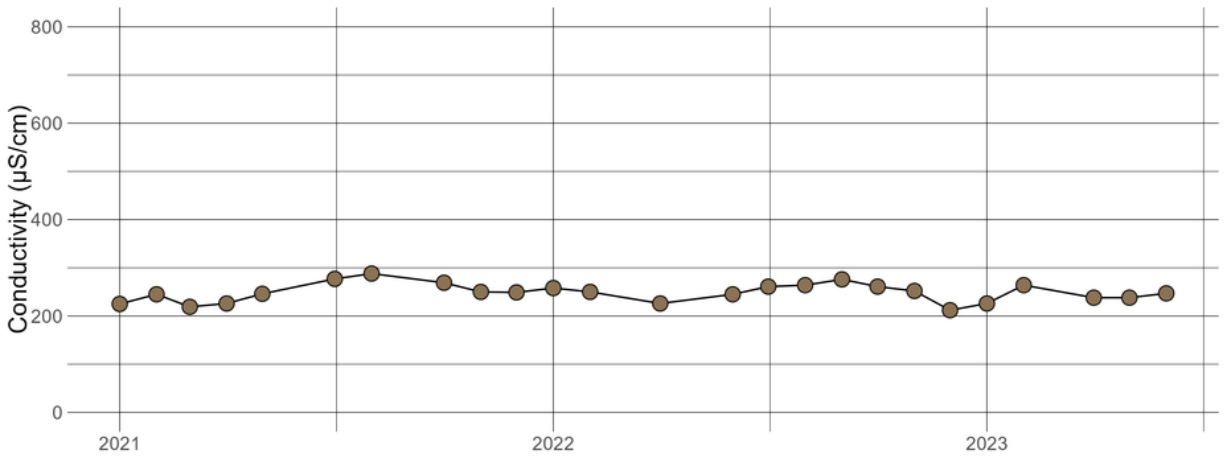
SOUBRACODCRE23.11 - Conductivity
