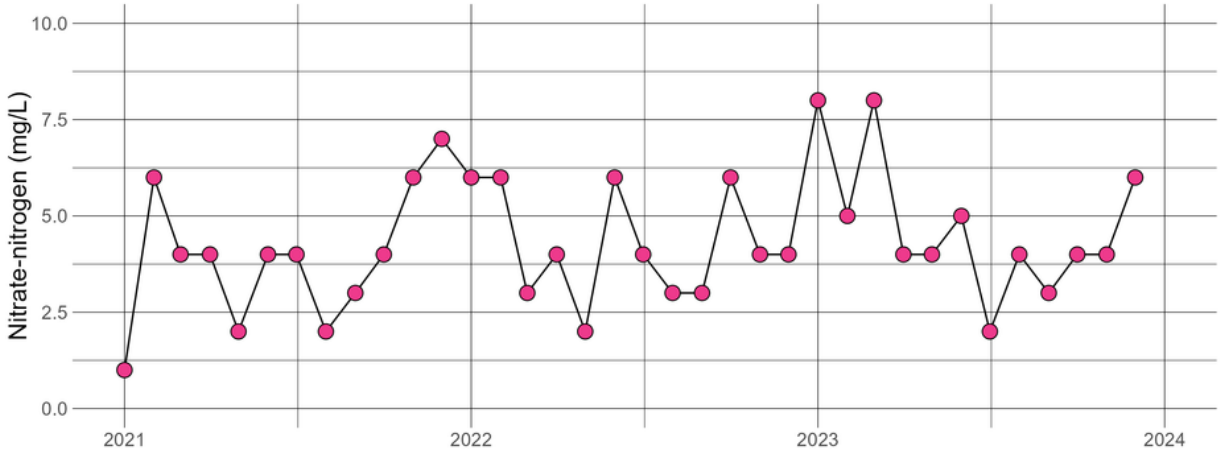
MUDCRE17.55 - Nitrate-nitrogen
