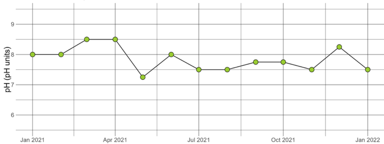
CONCRE2.81 - pH
