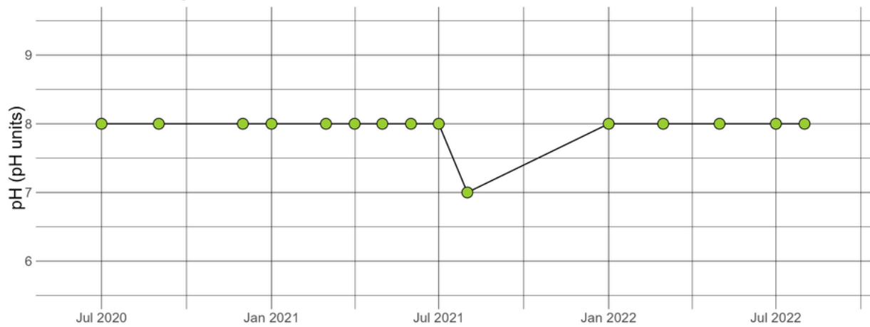
WILRUN0.37 - pH
