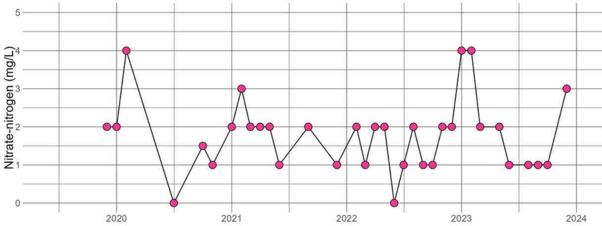
LITCONCRE12.56 - Nitrate-nitrogen
