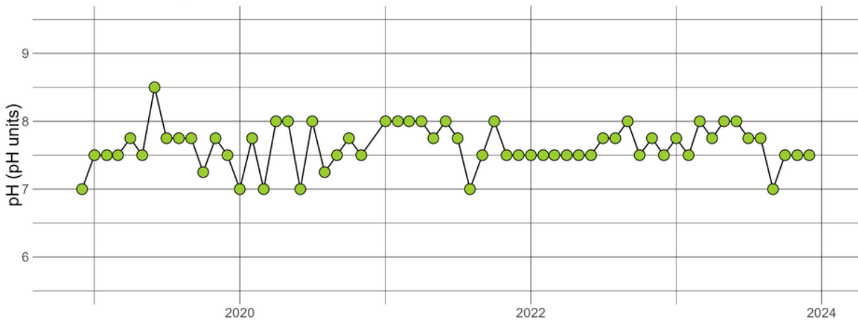
KRECRE8.67 - pH
