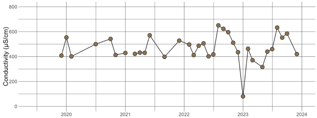
LITCONCRE12.56 - Conductivity
