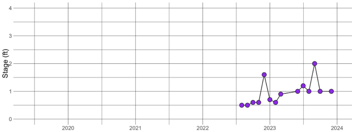
LITCONCRE12.56 - Stage
