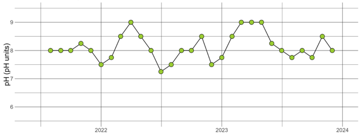
DOERUN1.77 - pH
