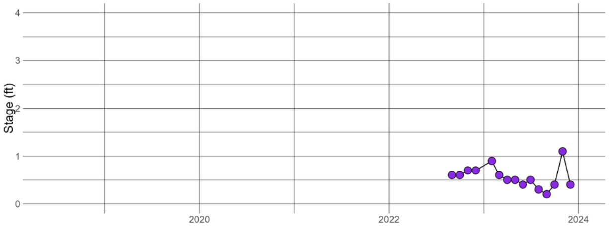
TYLRUN0.50 - Stage
