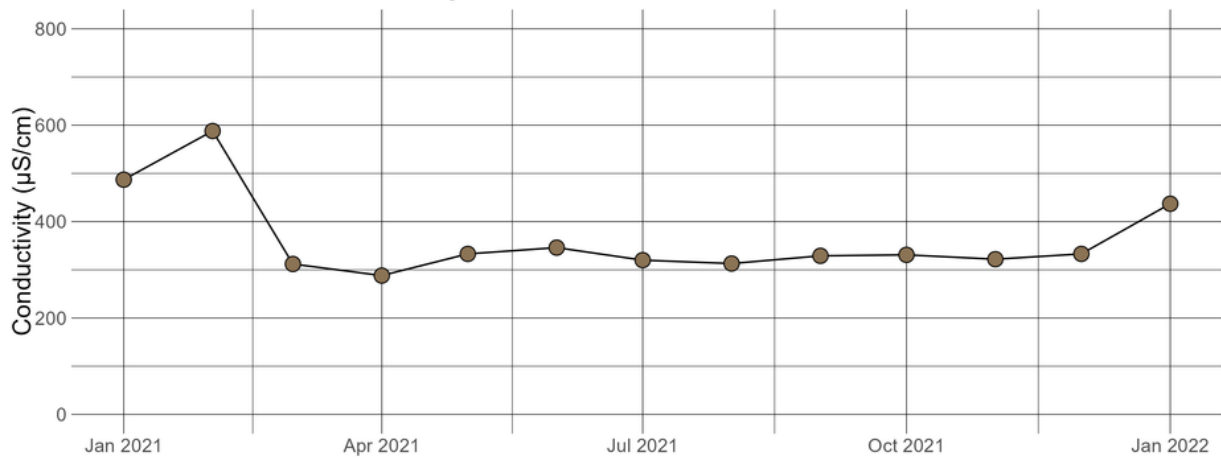
CONCRE2.81 - Conductivity
