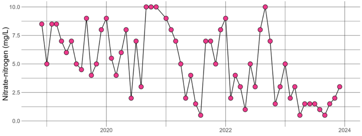
KRECRE8.67 - Nitrate-nitrogen
