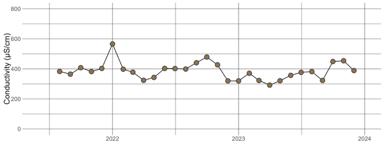
DOERUN1.77 - Conductivity
