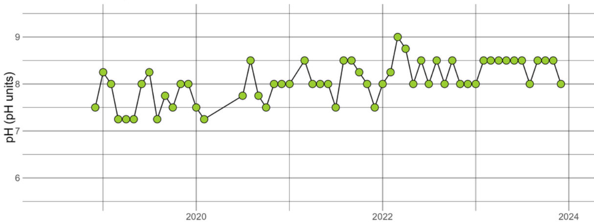
TYLRUN0.50 - pH
