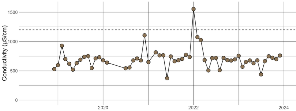
TYLRUN0.50 - Conductivity
