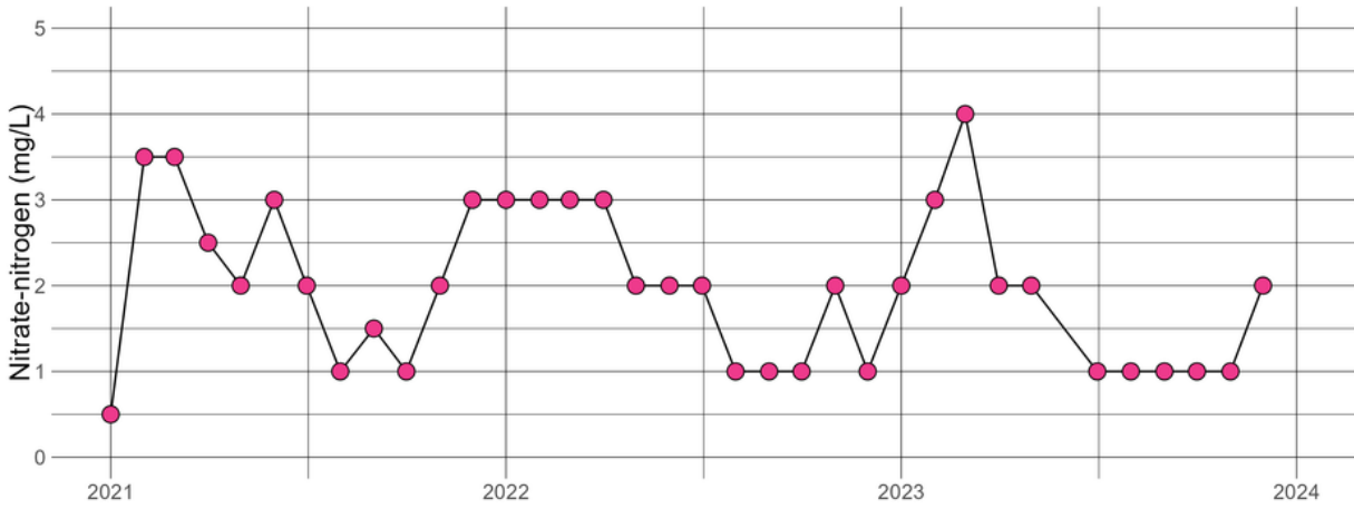
CODCRE5.77 - Nitrate-nitrogen
